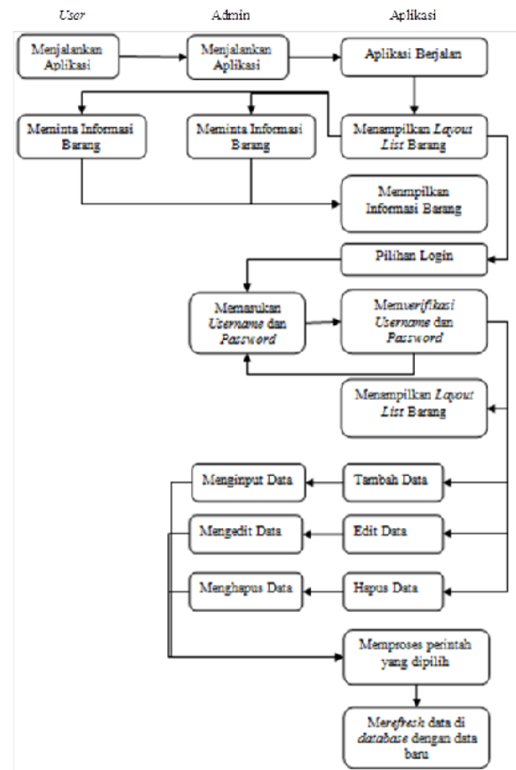
Gambar 5. Diagram Activity
